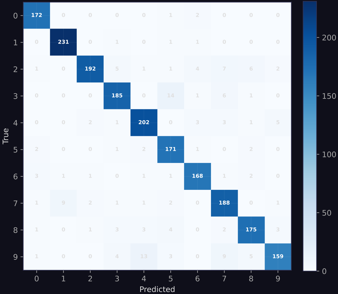
Confusion Matrix — Tuned SNN
