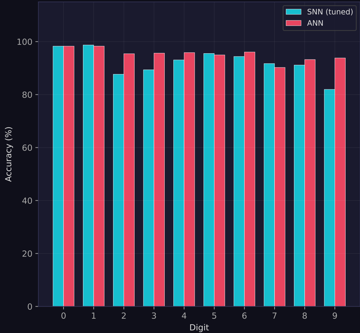
Per-Digit Test Accuracy
